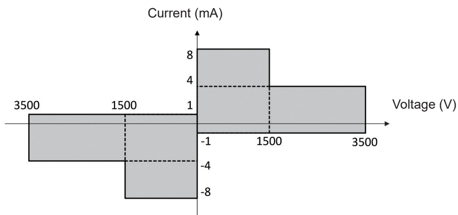
HVSMU Measurement and Output Range
