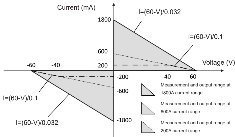
UHCU Measurement and Output Range
