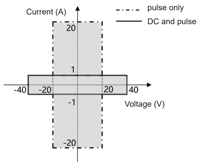
HCSMU Measurement and Output Range
