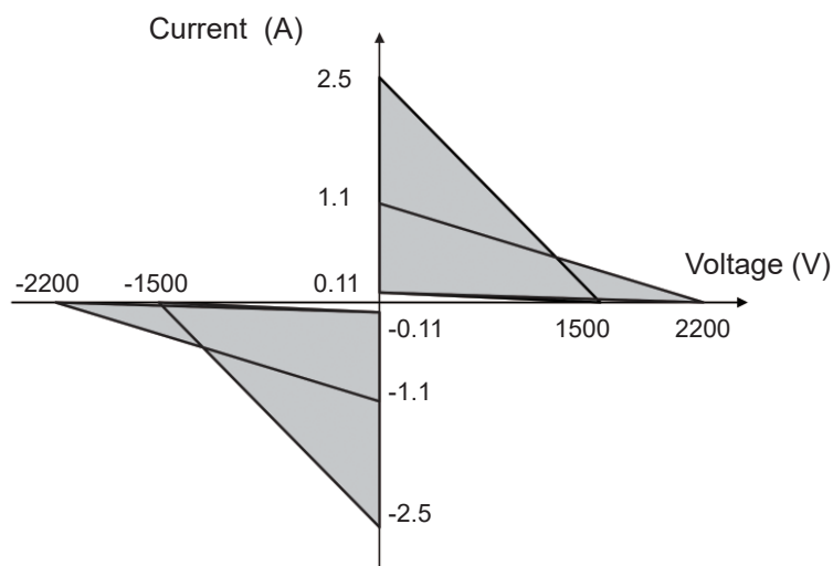
HVMCU Measurement and Output Range
