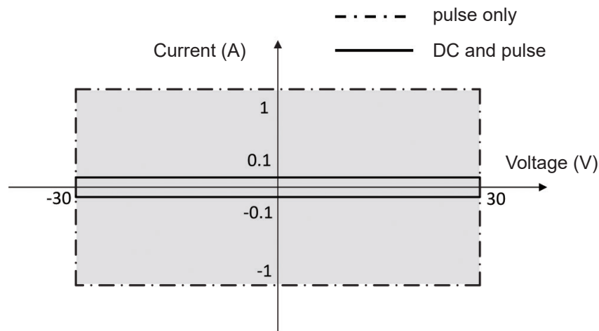
MCSMU Measurement and Output Range
